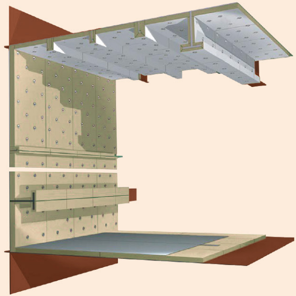
A-CLASS BULKHEAD & DECK
